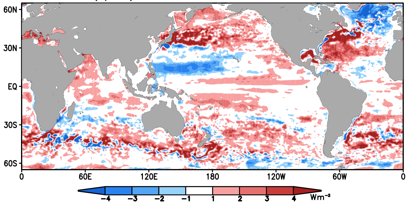
SODA4 (1/10°) 0–1000m HEAT STORAGE 2005–2023
