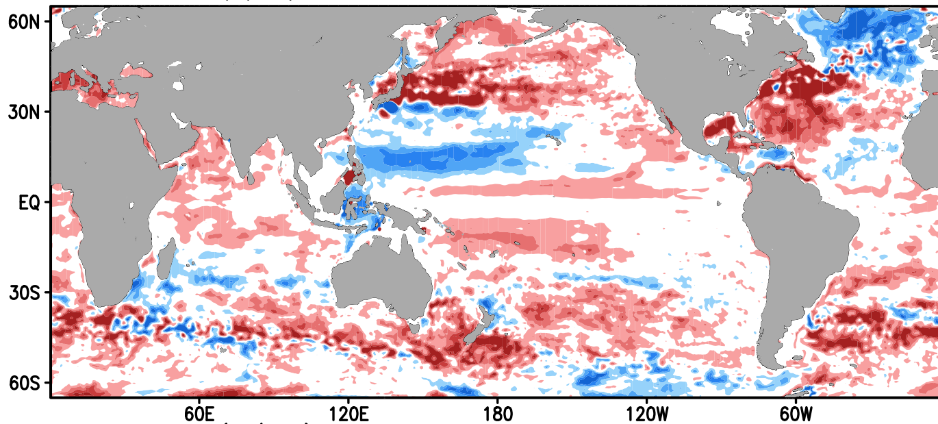
SODA4 (1/10°) 0–1000m HEAT STORAGE 2005–2023
